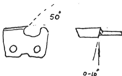
fig 7. 0-10° vinkel
